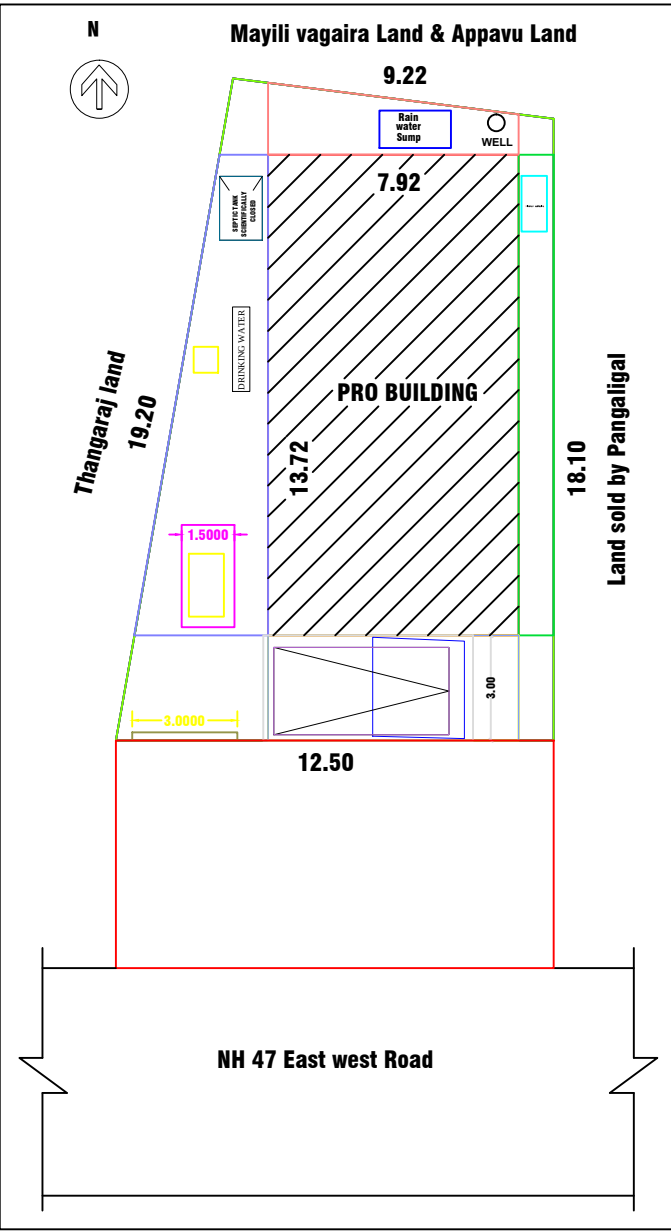
SITE PLAN & KEY PLAN
