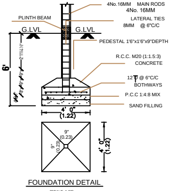
FOUNDATION DETAIL
