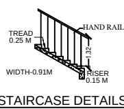
STAIRCASE DETAILS
