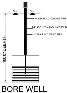
BORE WELL
