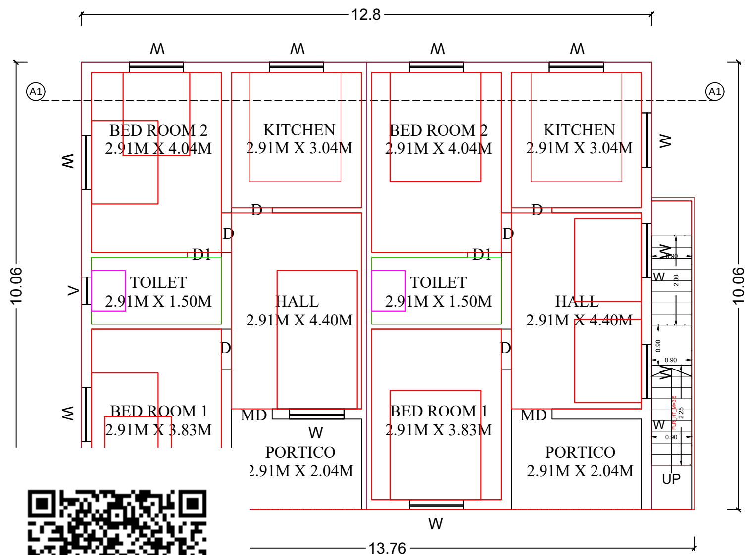
D FLOOR PLAN
