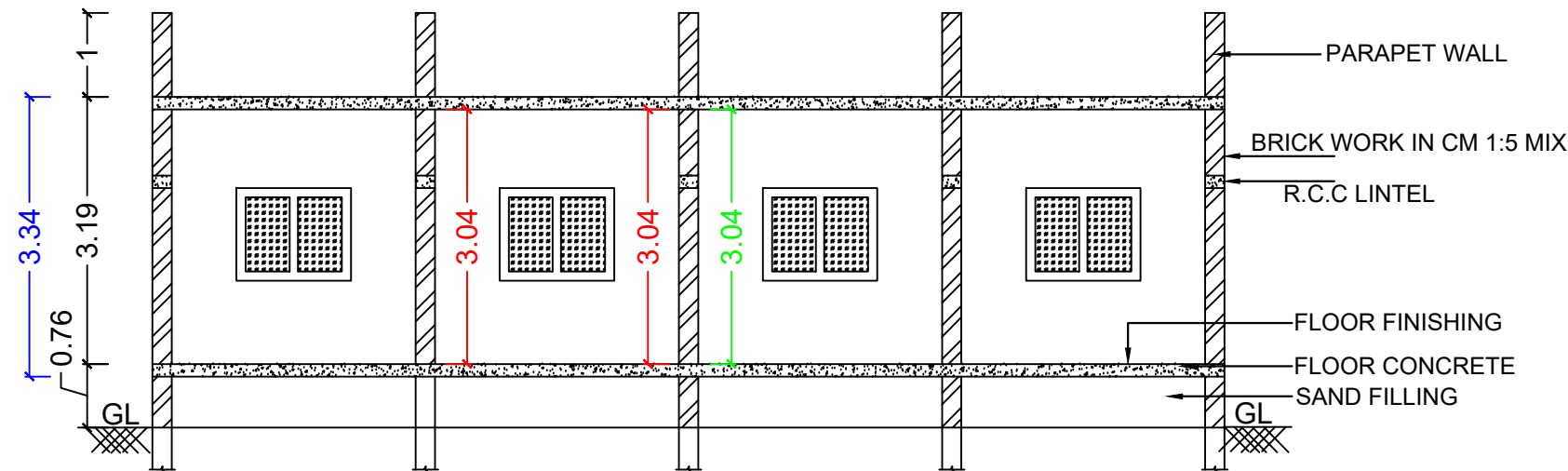
SECTION AT A1-A1
