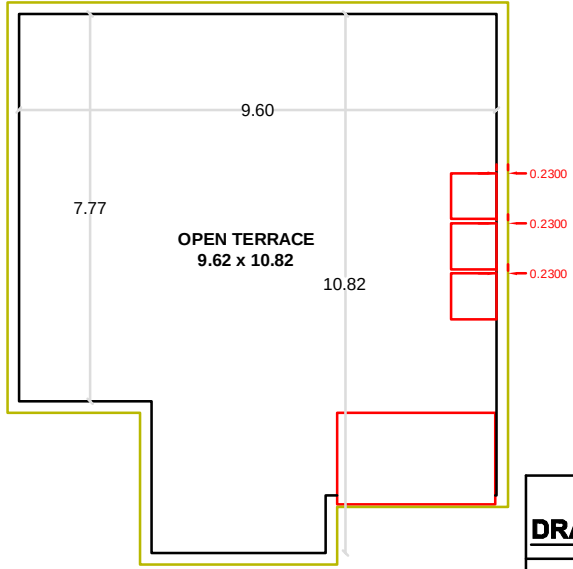
TERRACE PLAN PROPOSED
