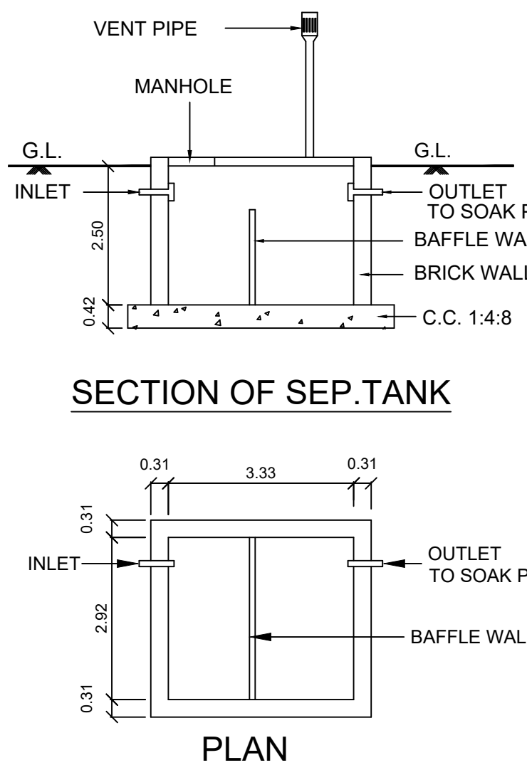
SEPTIC. TANK
