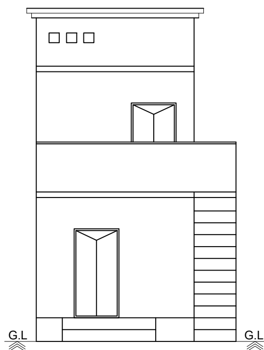
FRONT ELEVATION
