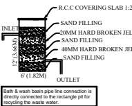
Waste Water Recycle Unit Not To Scale
