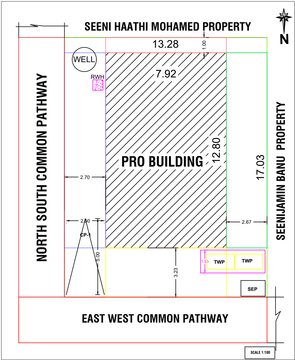
SITE PLAN
