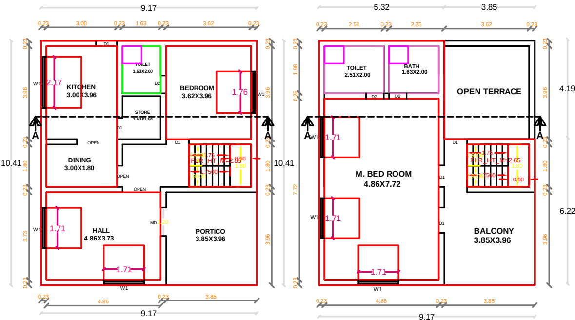
GROUND FLOOR PLAN PROPOSED
