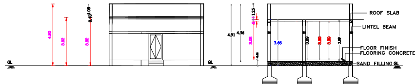
FRONT ELEVATION
