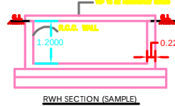
RWH_CAPACITY_L=2000LTRS
