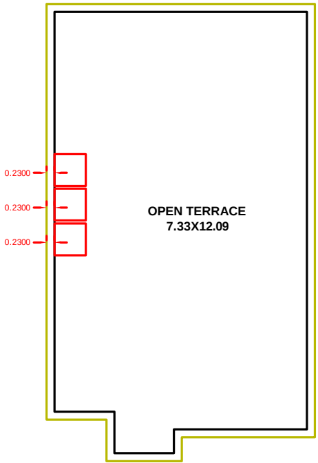
TERRACE FLOOR PLAN PROPOSED
