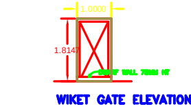
WIKET GATE ELEVATION
