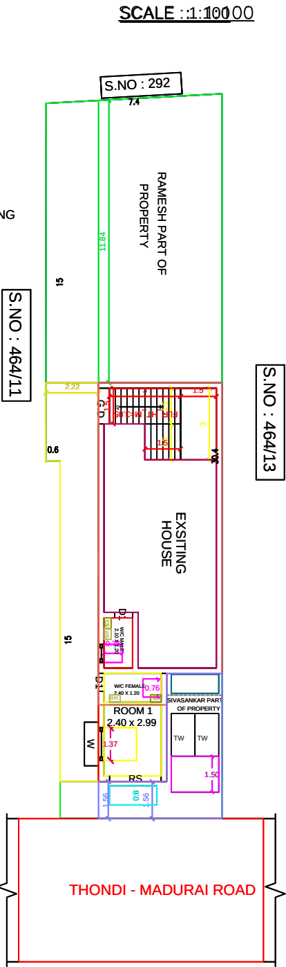
SITE PLAN CUM PROPOSED GROUND FLOOR PLAN
