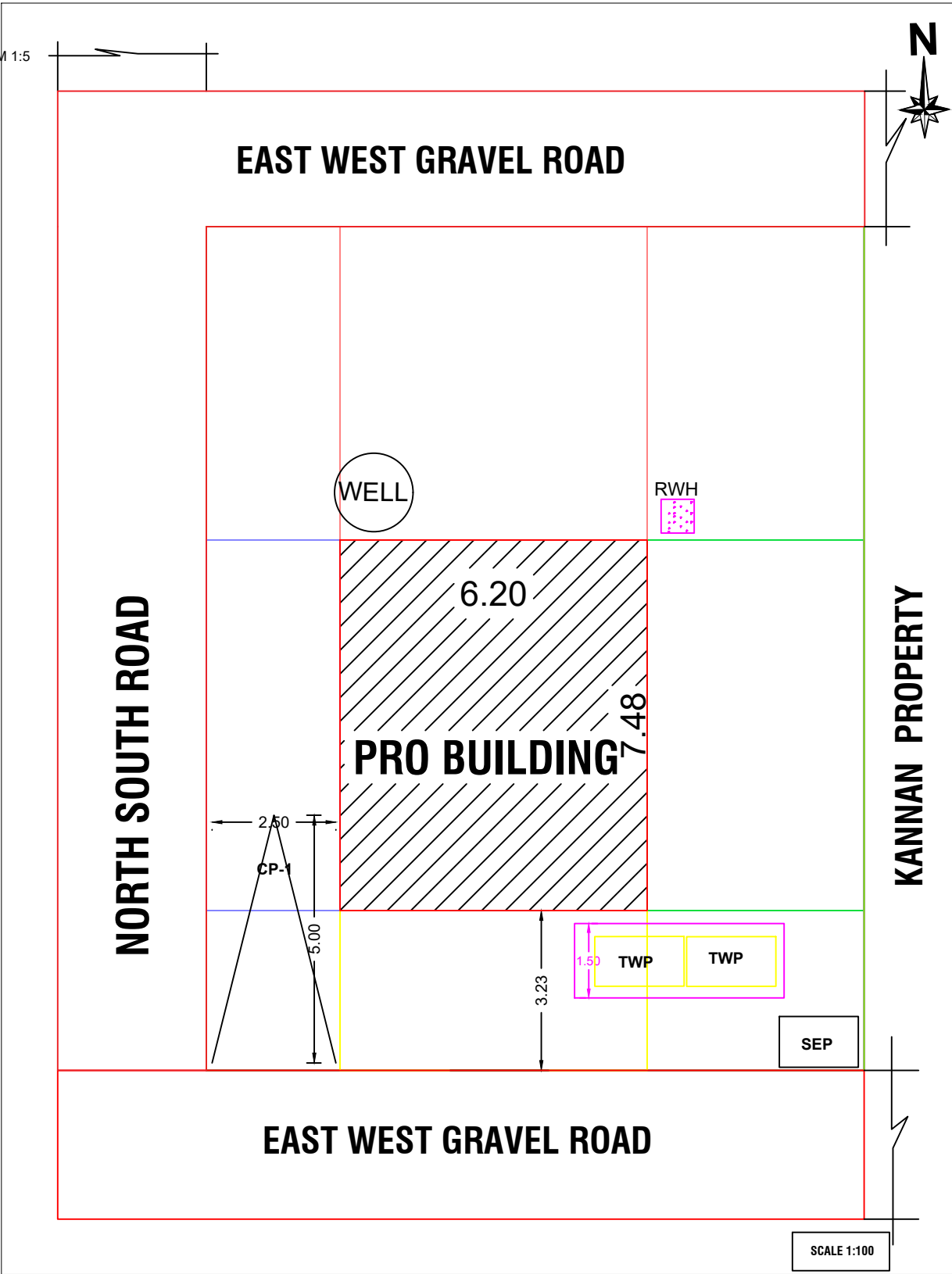
SITE PLAN
