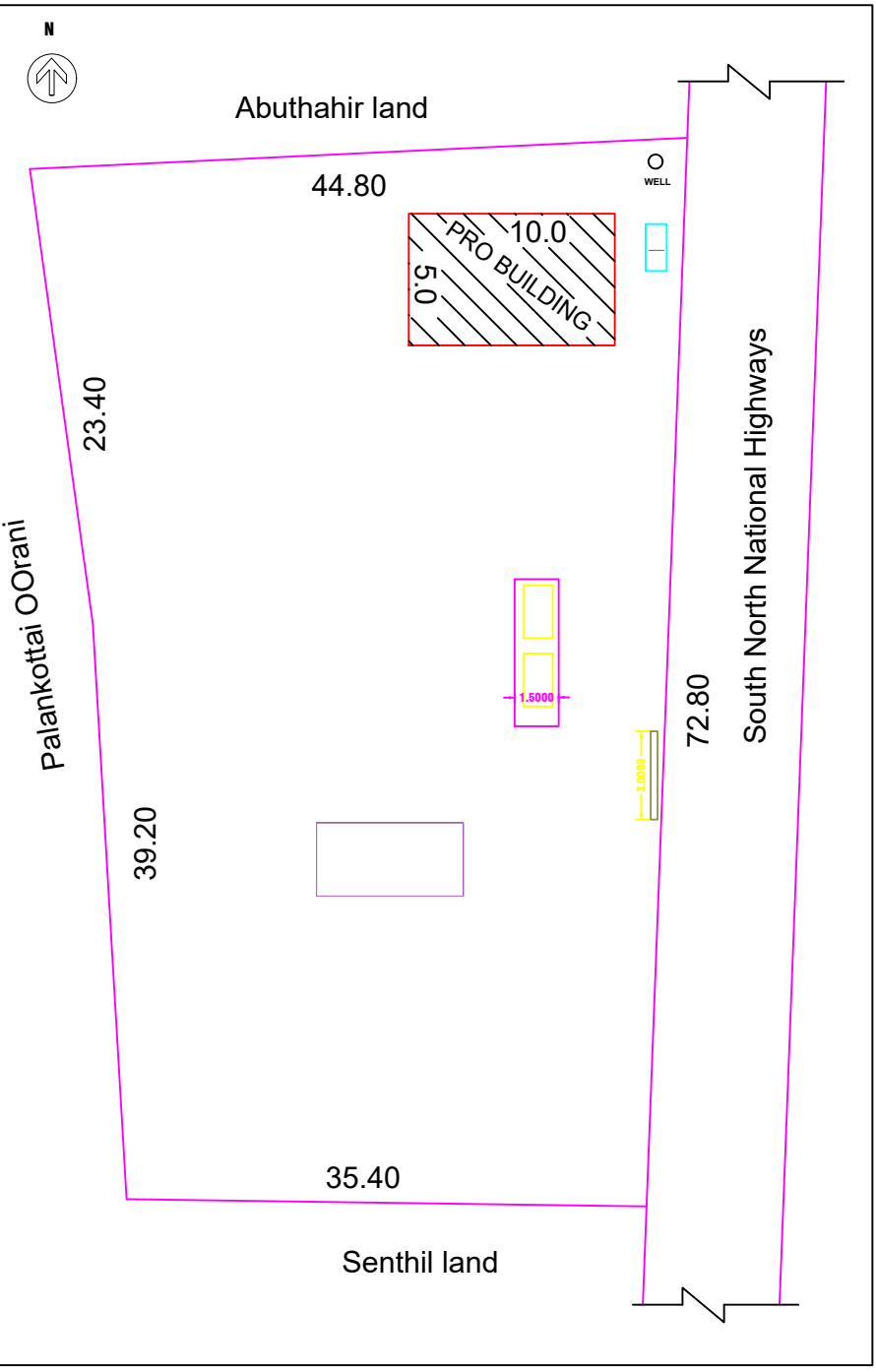
SITE PLAN & KEY PLAN
