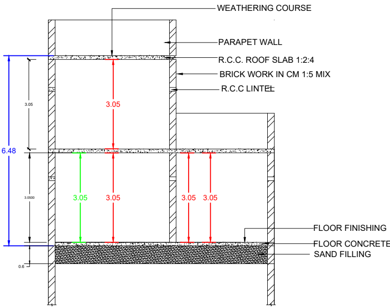
SECTION A1-A1
