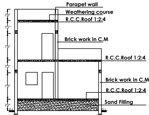
SECTION ON XX
