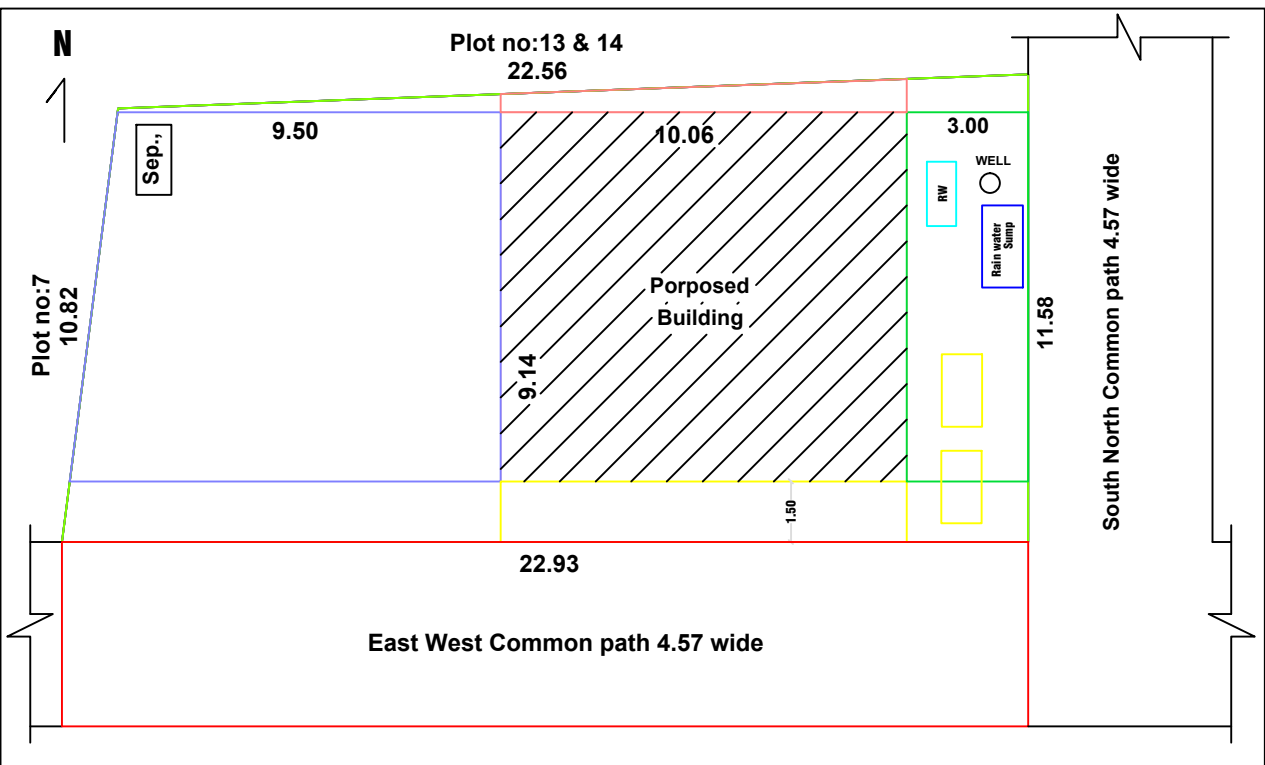
SITE PLAN CUM KEYPLAN
