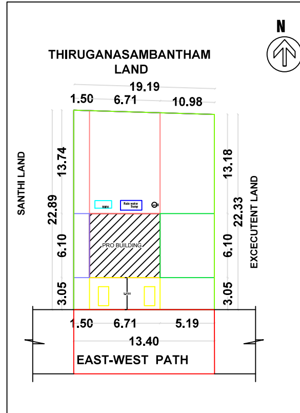
SITE PLAN & KEY PLAN
