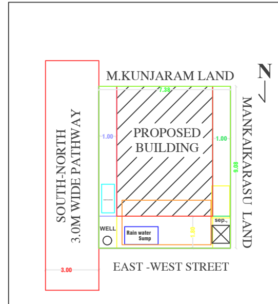
SITE PLAN CUM KEYPLAN
