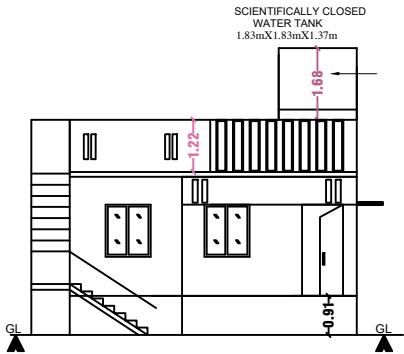
FRONT ELEVATION
