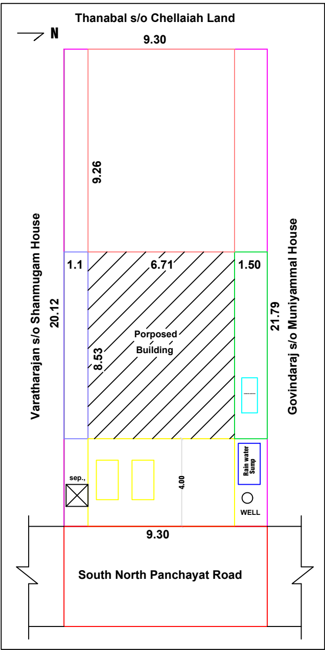
SITE PLAN CUM KEYPLAN
