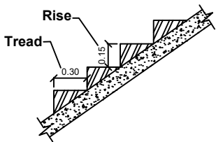
STAIRCASE DETAILS
