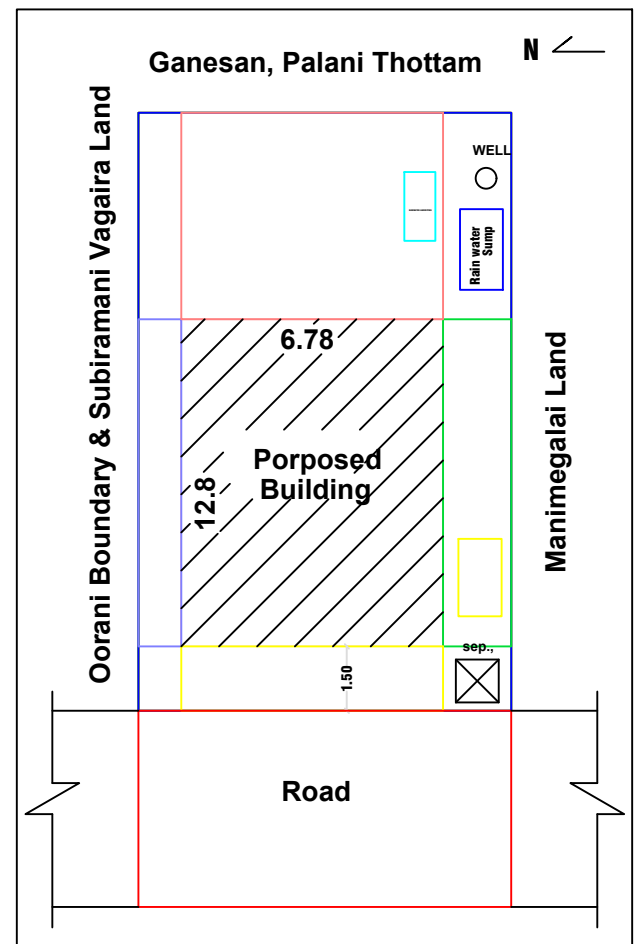
SITE PLAN CUM KEYPLAN
