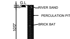
PERCOLATION PIT
