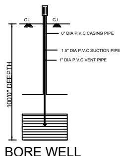
BORE WELL
