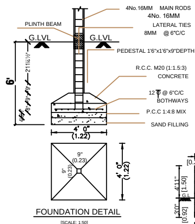
SECTION - CC
