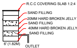
wash basin pipe line connection is connected to the rectangle pit for ng the waste water.
