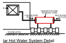
Hot Water System Detail
