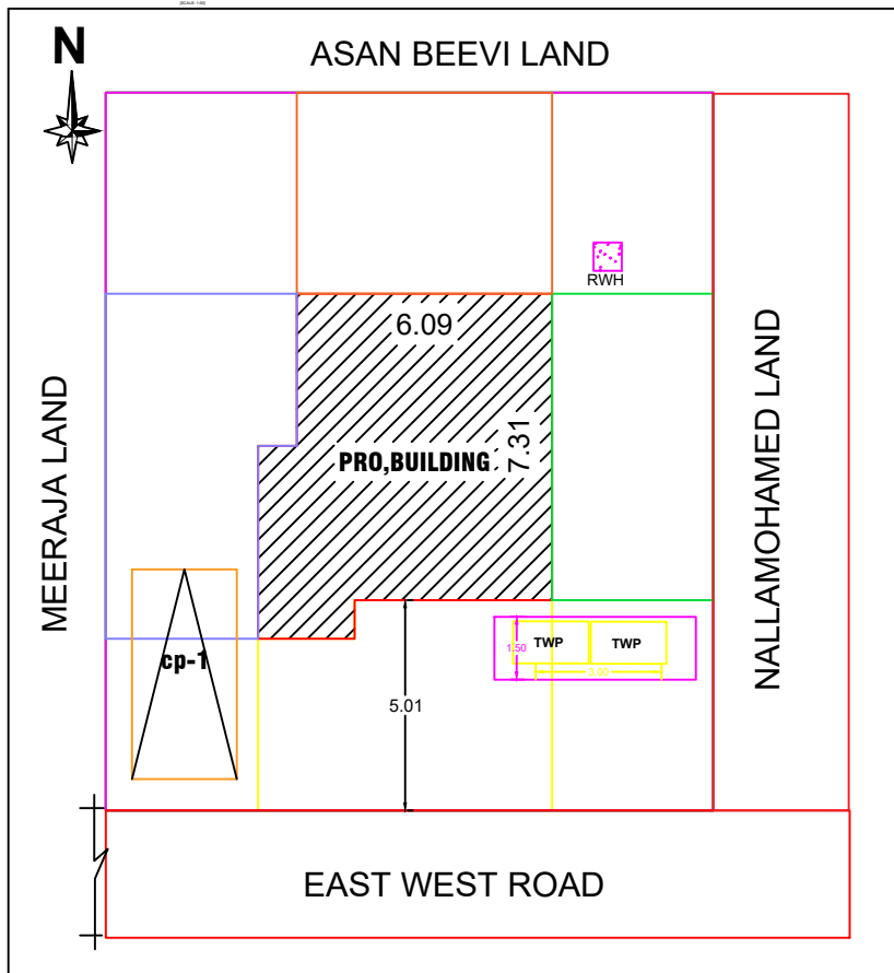
SITE PLAN
