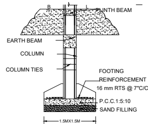
FOUNDATION DETAIL
