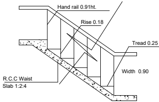
STAIRCASE DETAIL
