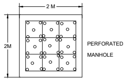
PLAN OF RAIN WATER RECHARGING PIT
