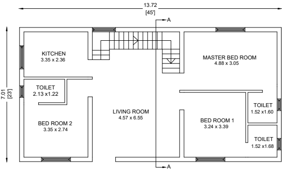
EXG. GROUND FLOOR PLAN
