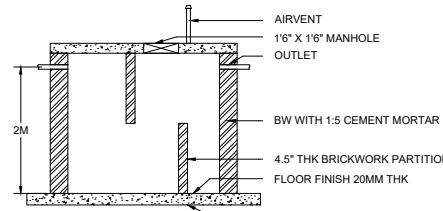
CROSS SECTION OF SEPTIC TANK
