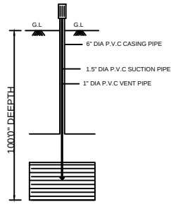
BORE WELL
