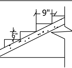
Staircase Detail Not To Scale
