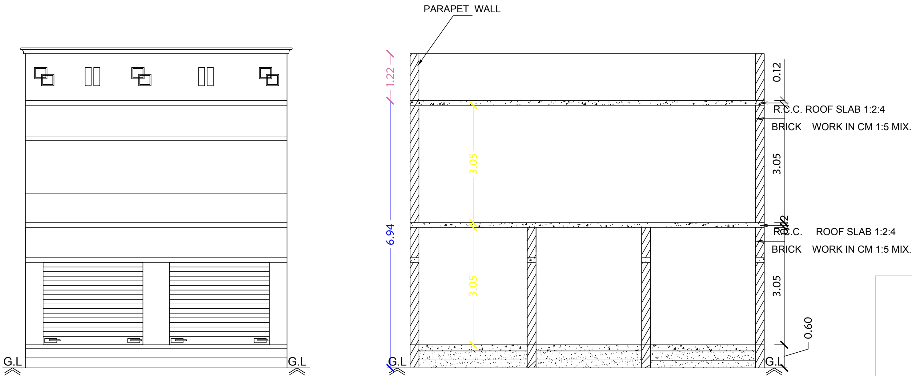
Front Elevation
