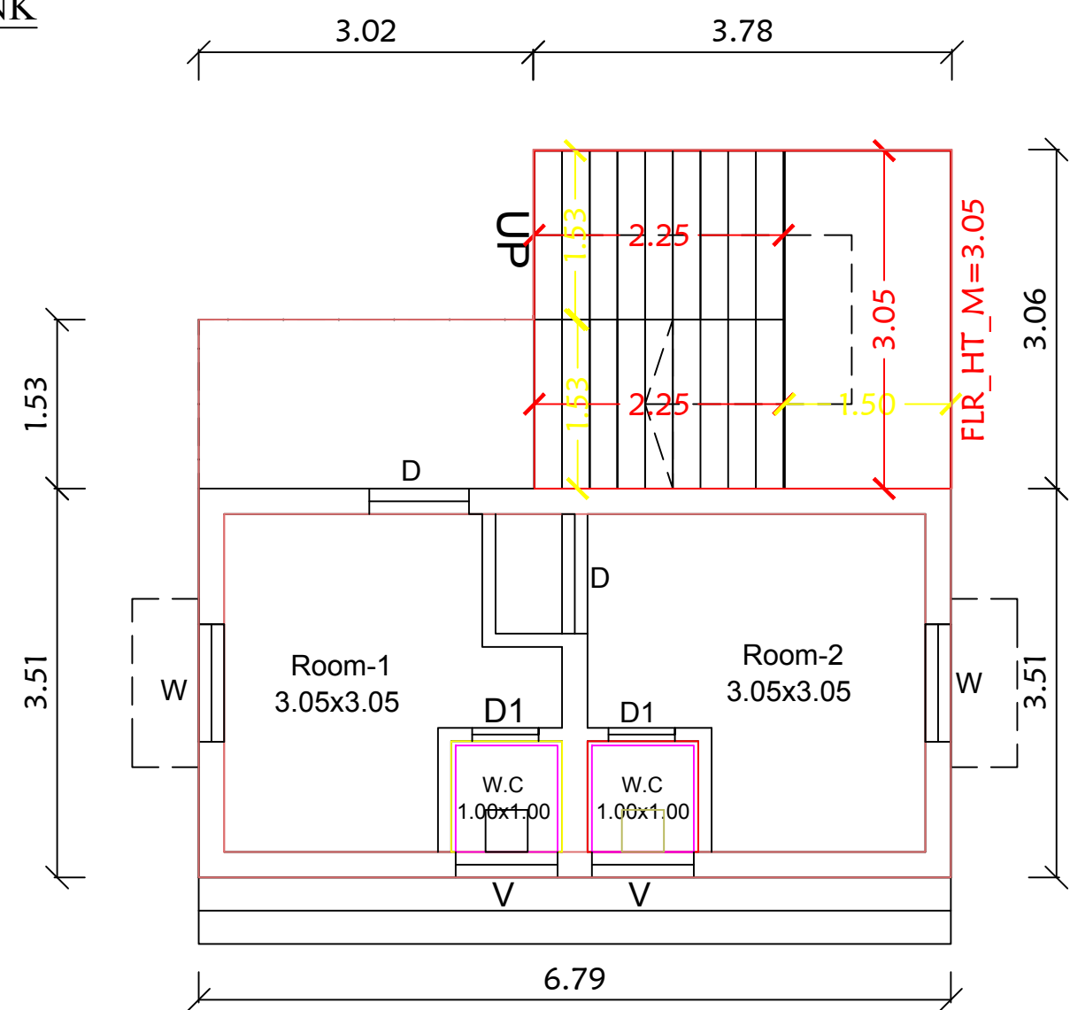
First Floor
