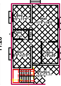
EXISTING GROUND FLOOR
