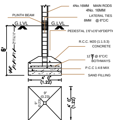
FOUNDATION DETAIL
