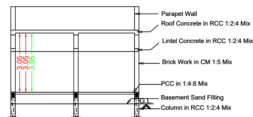
Section RR
