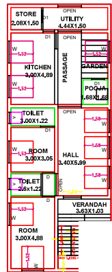
GROUND FLOOR
