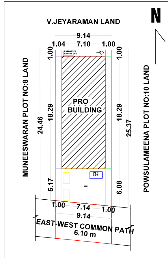
SITE PLAN & KEY PLAN (1:100)
