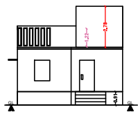
FRONT ELEVATION 7.10
