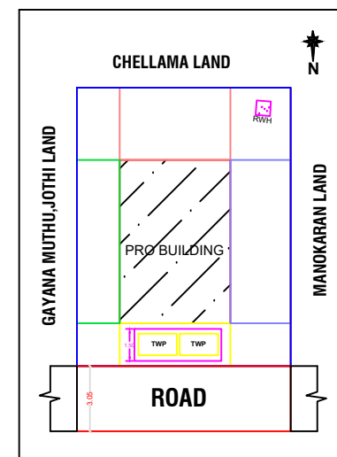
SITE PLAN
