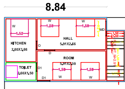
FIRST FLOOR PLAN ( RESIDENTIAL )
