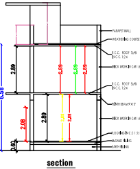
section
