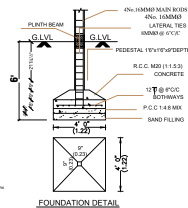
FOUNDATION DETAIL
