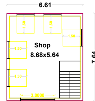
PRO. GROUND FLOOR PLAN
