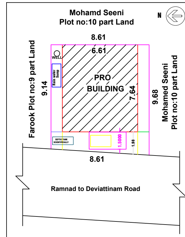
SITE PLAN & KEY PLAN
