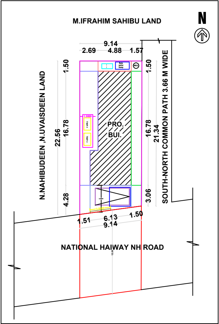
SITE PLAN & KEY PLAN
