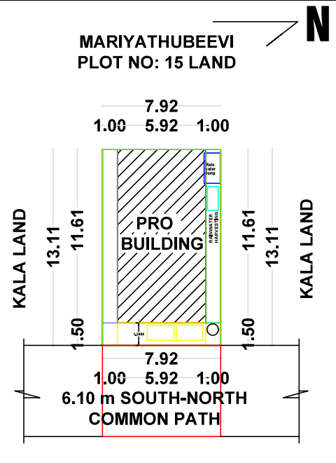
SITE PLAN & KEY PLAN (1:100)
