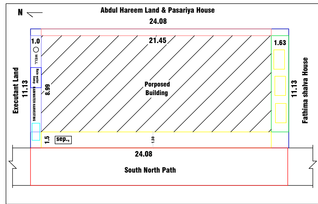
SITE PLAN CUM KEYPLAN
