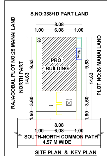
SITE PLAN & KEY PLAN
