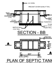
PLAN OF SEPTIC TANK
