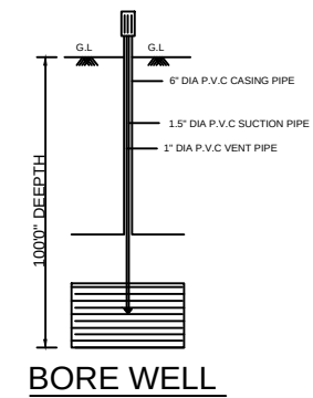
FOUNDATION DETAIL
