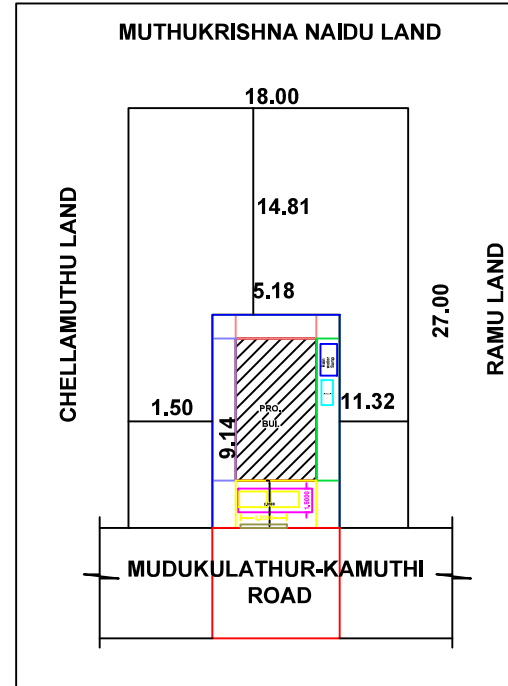
SITE PLAN & KEY PLAN
