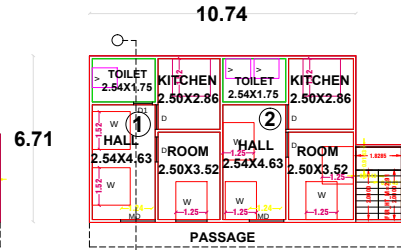
PROPOSED SECOND FLOOR PLAN
