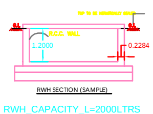
RWH SECTION (SAMPLE)
