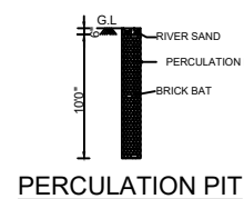
PERCULATION PIT
