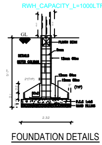
FOUNDATION DETAILS
