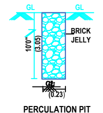
PERCULATION PIT
