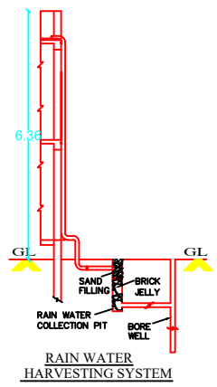
RAIN WATER HARVESTING SYSTEM
