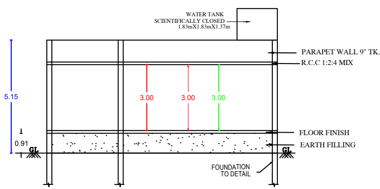
SECTION AB
