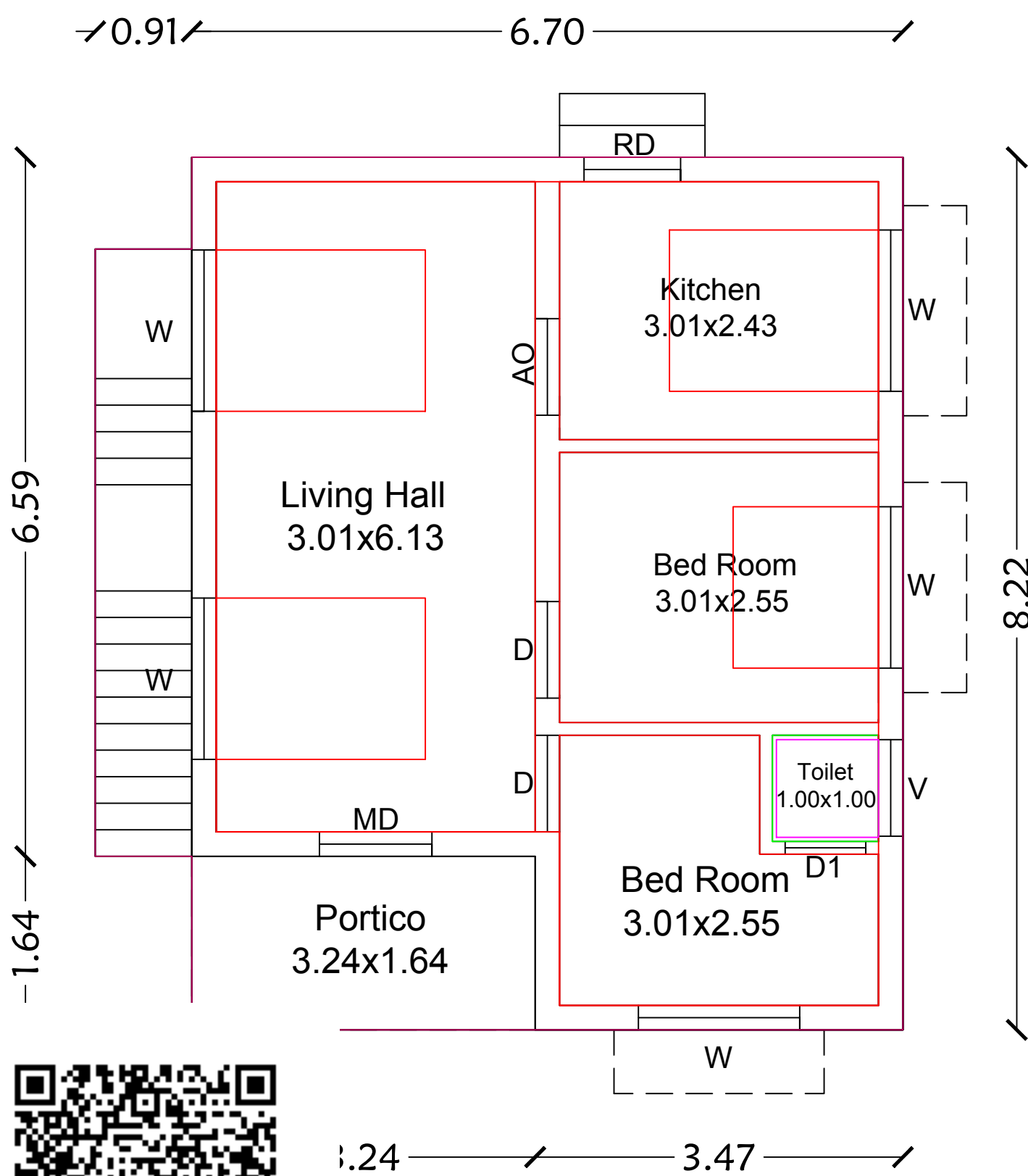
round Floor
