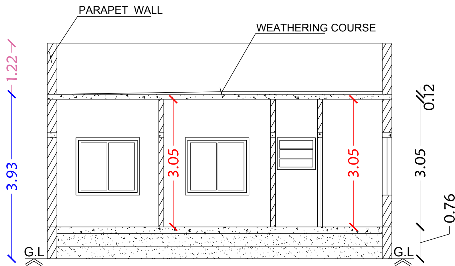
Section on-"AA"
