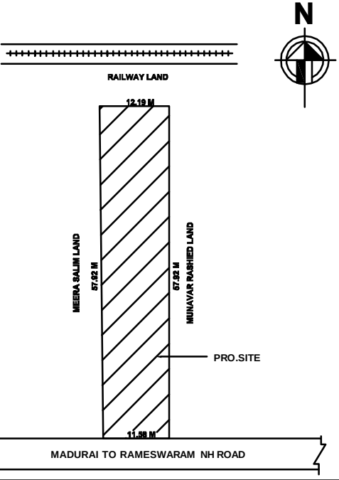
LOCATION PLAN
