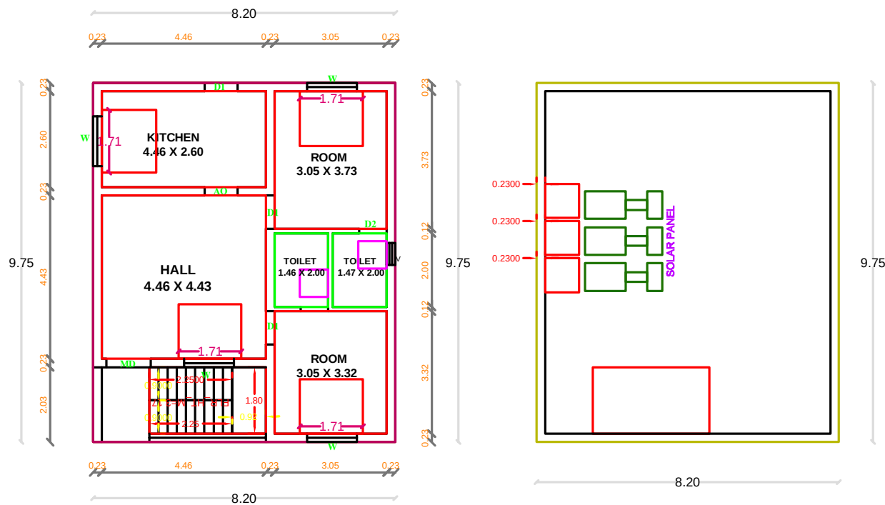
GROUND FLOOR PLAN PROPOSED
