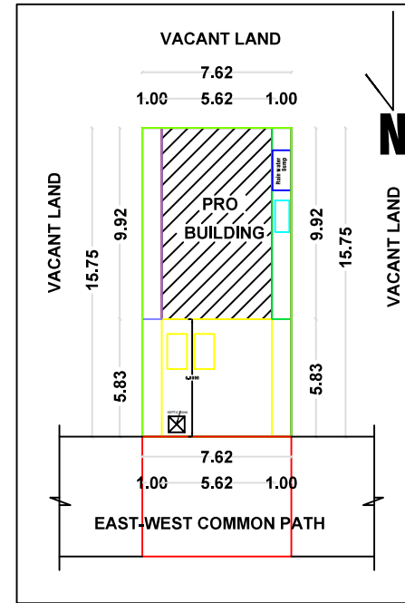
SITE PLAN & KEY PLAN
