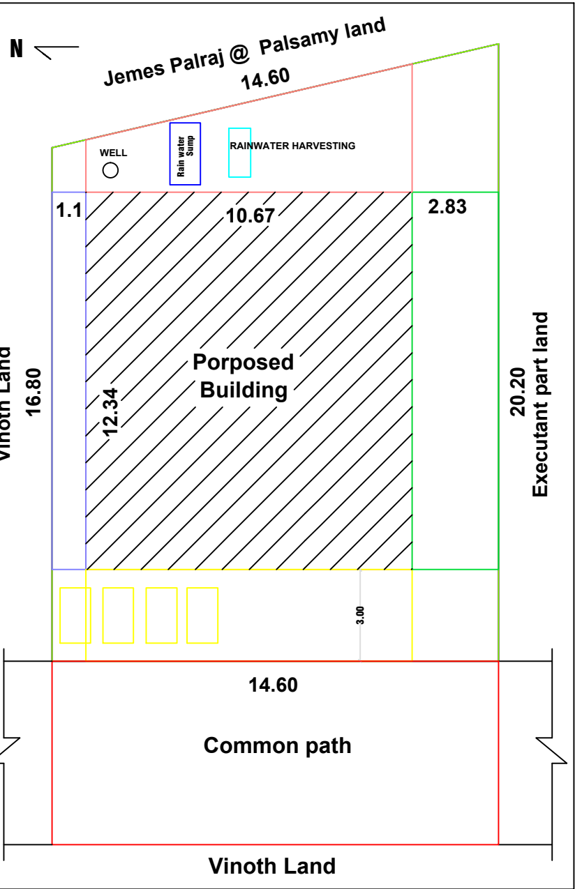
SITE PLAN CUM KEYPLAN
